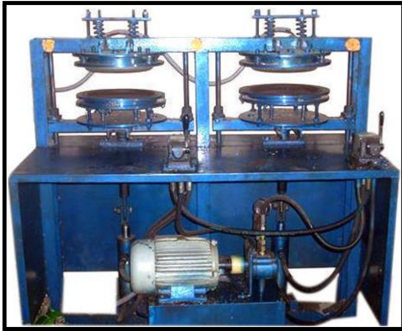
Automatic Paper Plate Making Machine
